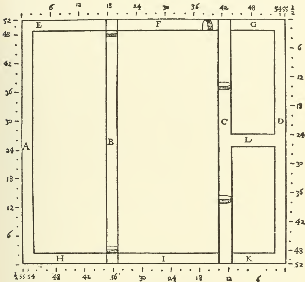
THE FOUR LONG WALLS: A—FIRST. B—SECOND. C—THIRD. D—FOURTH. THE SEVEN TRANSVERSE WALLS: E—FIRST. F—SECOND. G—THIRD. H—FOURTH. I—FIFTH. K—SIXTH. L—SEVENTH, OR MIDDLE.
